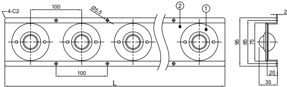
Model: 25BCR25 Ball Ø25.4mm (1")
