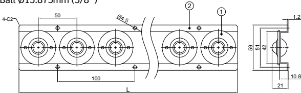
Model: 25BCR16 Ball Ø15.875mm (5/8")
